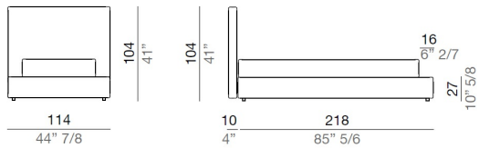
Single Bed 114 cm, base 82x202 cm - L114
