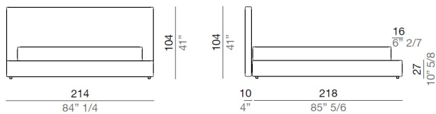
Double Bed 214 cm, base 182x202 cm - L214
