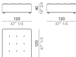
Seat Element 120 cm - PF120
